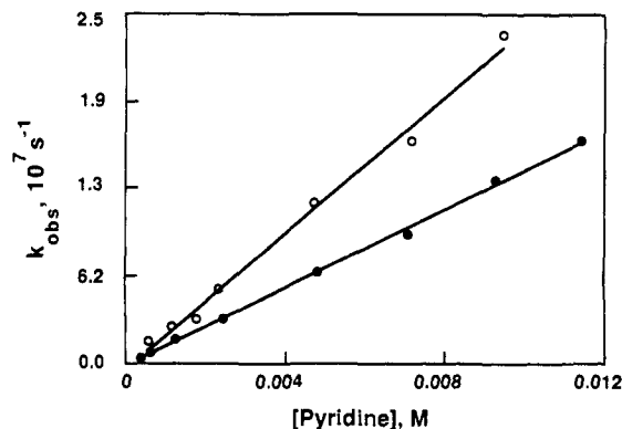
Figure 5. Observed rate constant for growth of the pyridine ylide derived from DNQ-4Ph (○) and DNQ-5Ph (●) in ACN as a function of pyridine concentration.
